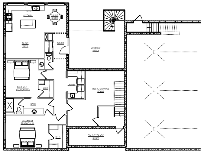
*** LEGAL SUITE PLAN 9' 3" FOUNDATION WALL HEIGHT
