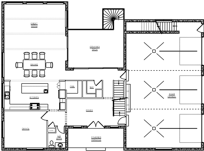
MAIN FLOOR PLAN 9'-11" WALL HEIGHT
