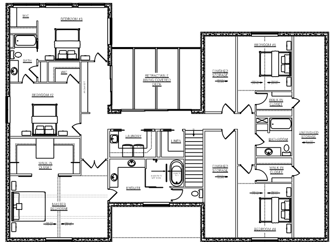
SECOND FLOOR PLAN 9' 1" WALL HEIGHT
