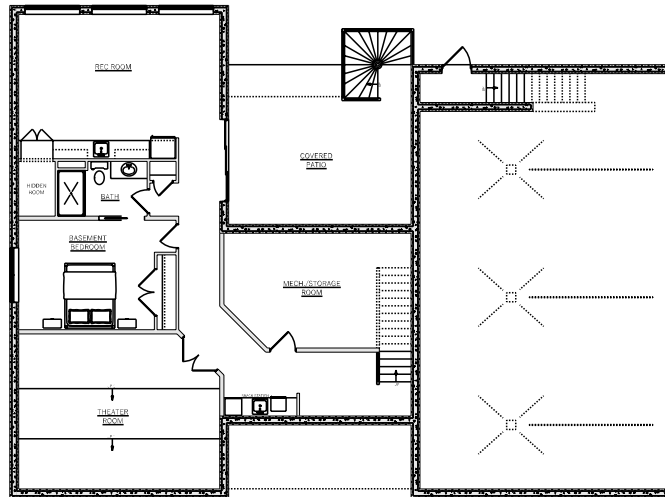
BASEMENT DEV. PLAN 8' 3" FOUNDATION WALL HEIGHT
