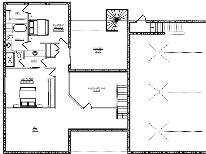
*** BASEMENT DEV. PLAN 9'-3" FOUNDATION WALL HEIGHT
