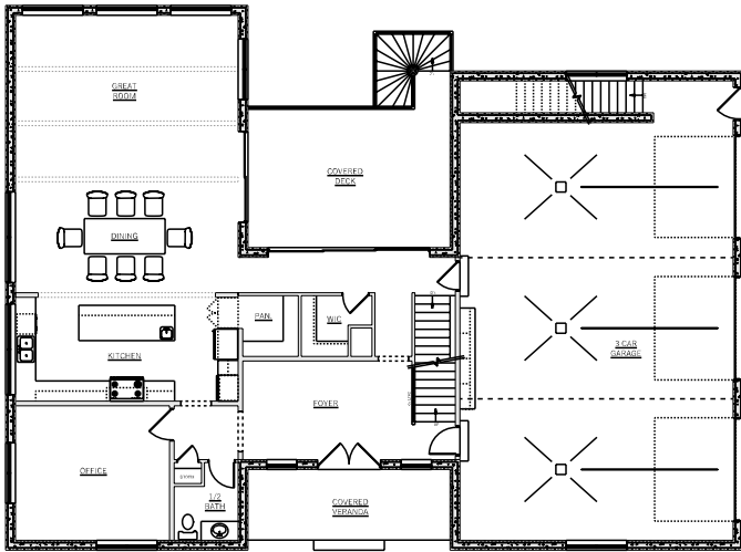
MAIN FLOOR PLAN 9'-10" WALL HEIGHT
