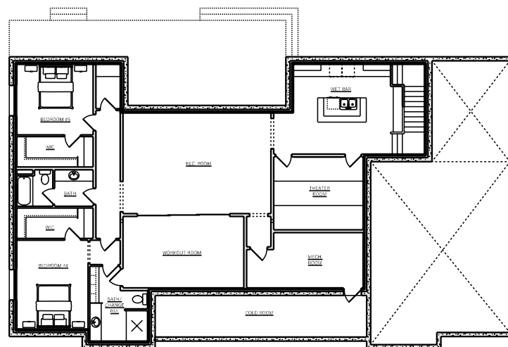
BASEMENT DEV. PLAN 9'-0" FOUNDATION WALL HEIGHT
