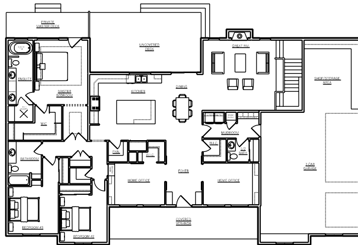
MAIN FLOOR PLAN 9'-1" WALL HEIGHT
