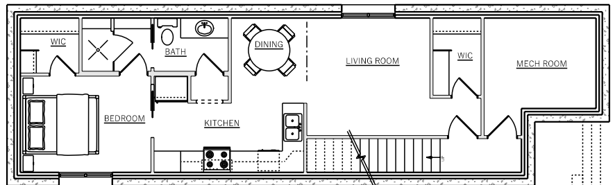
LEGAL BASEMENT PLAN 8' 9" WALL HEIGHT
