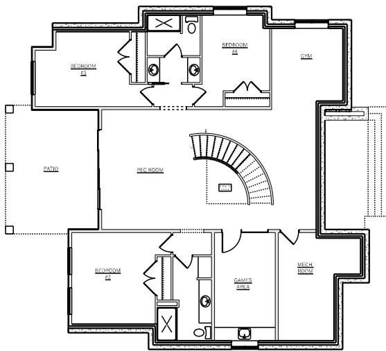
BASEMENT DEV. PLAN 9'-4" FOUNDATION WALL HEIGHT
