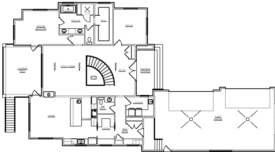
MAIN FLOOR PLAN 10'-1" WALL HEIGHT
