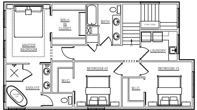
SECOND FLOOR PLAN 9' 1" WALL HEIGHT
