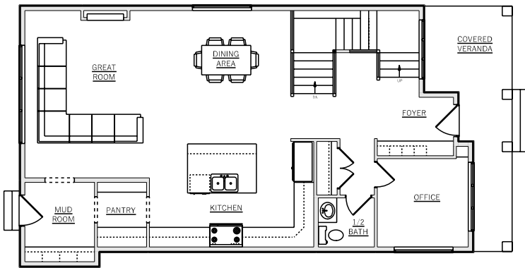
MAIN FLOOR PLAN 10' 1" WALL HEIGHT
