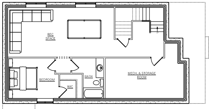
BASEMENT DEV. 9'-0" FOUNDATION WALL HEIGHT
